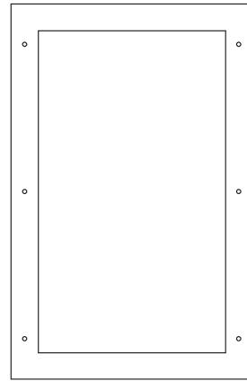
Trim Ring for APLI-16: Part No. 78001659
