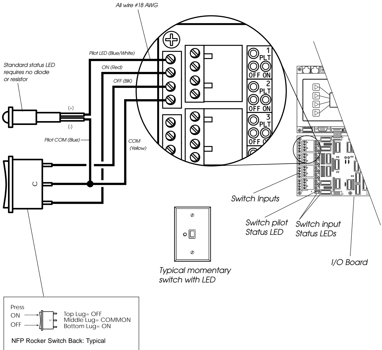
Typical Momentary NFP Switch Wiring
