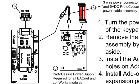
BACnet-MSTP Serial Interface module shown BACnet-IP and LonWorks modules have the same basic footprint
