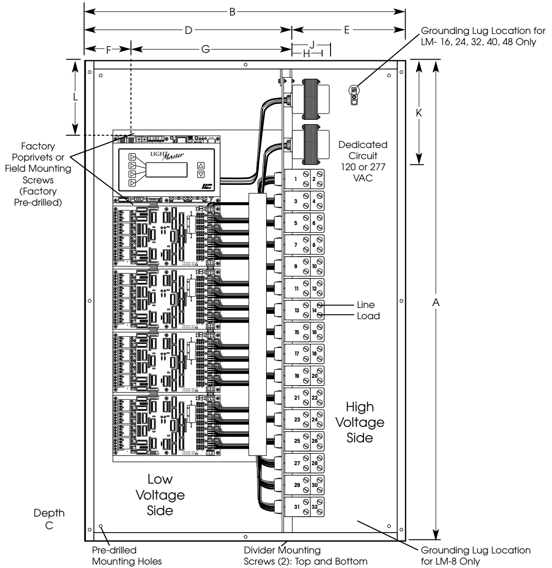
LightMaster 24/32 Layout Shown as Example NEMA-1 Type Enclosure (Custom enclosures available on request)
