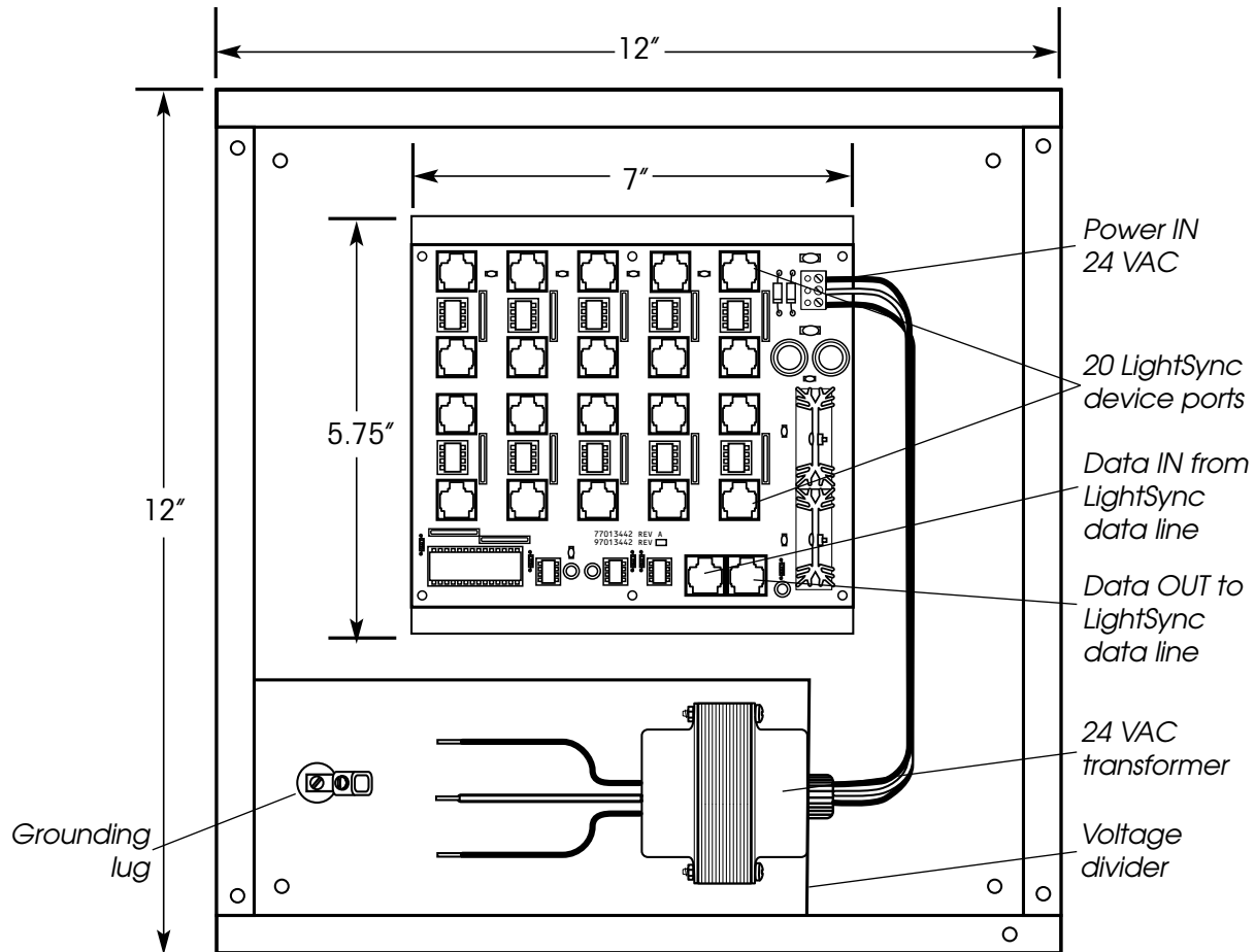
LightSync 20-port Hub (shown in optional enclosure with transformer)
