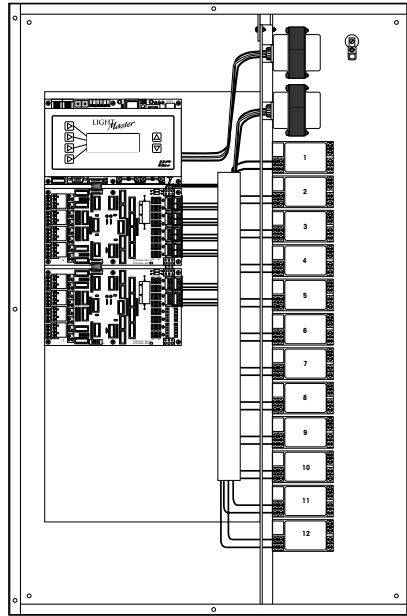
LightMaster 16 I/O processor in 24 size Enclosure w/ 12- 2PC relays
