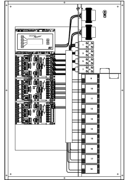
LightMaster 24 I/O processor in 24 size Enclosure w/ 8-2R9C and 10-2PC relays
