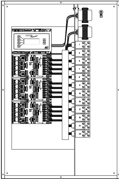
LightMaster 24 I/O processor in 24 size Enclosure w/ 24- 2R9C relays
