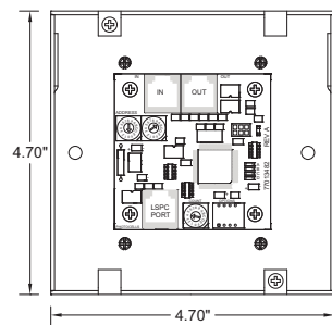
Remote Mount LSPSCAM-R
