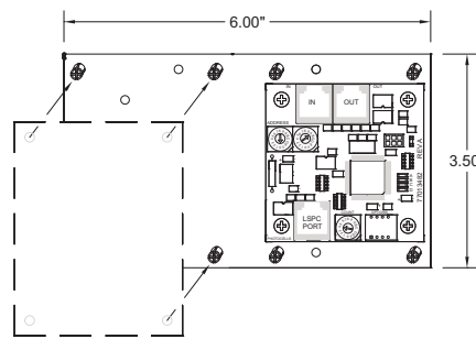
LSPSCAM-PR-P Panel Mount 2-Device Plate (Shown with space for optional modules)
