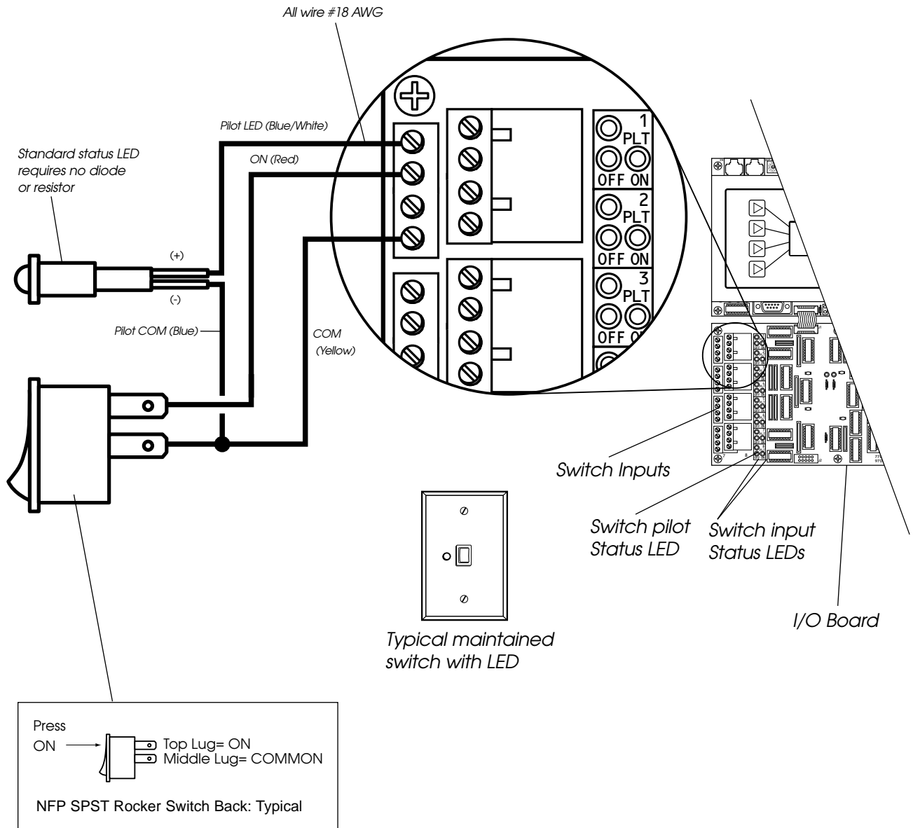
Typical Maintained NFP Switch Wiring
