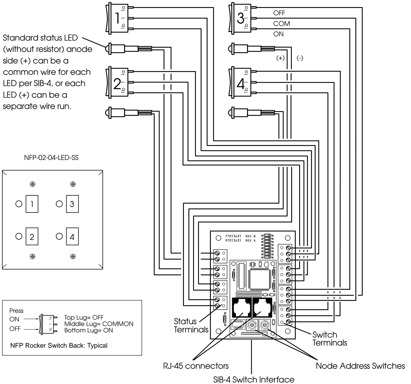
Typical Switch to SIB-4 Wiring
