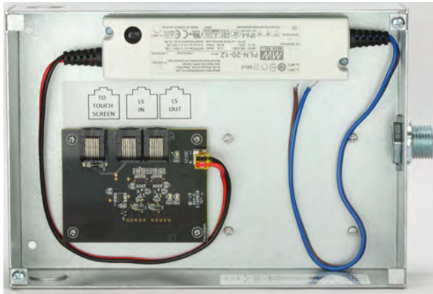
Figure 12 TSPI Power Injector enclosure
