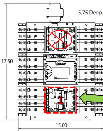
LightLEEDer-24 Retrofit Insert
