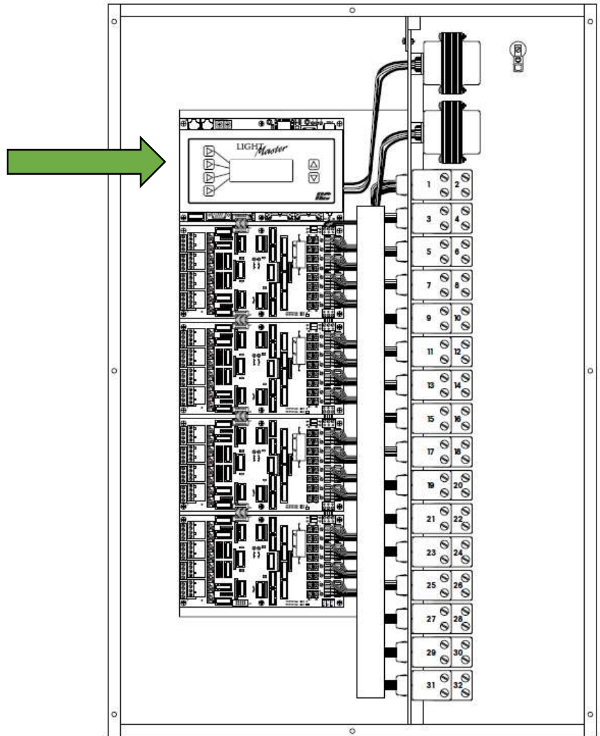
LightMaster 32 relay panel
