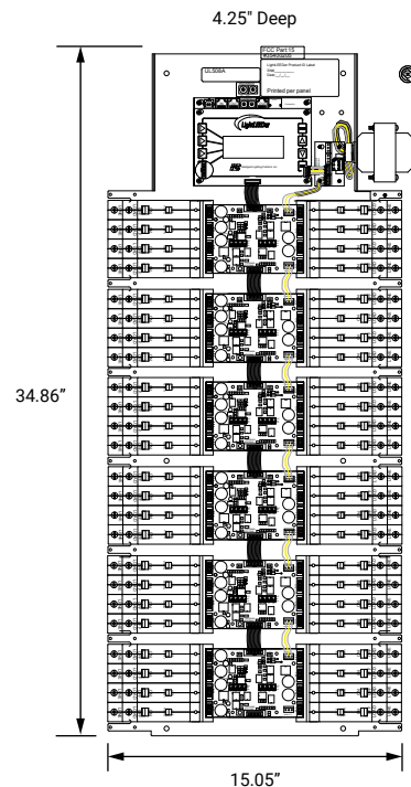
LLCD-48 Retrofit Insert (Enclosure: 37.5"H x 20"W x 6"D)
