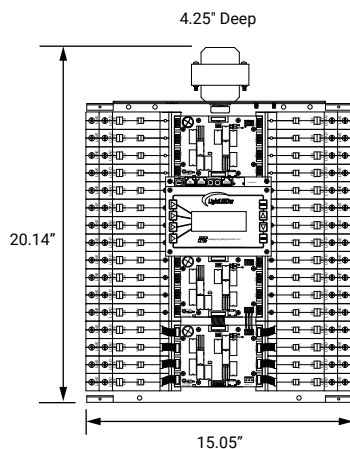
LLCD-32 Retrofit Insert (Enclosure: 25.5"H x 20"W x 6"D)
